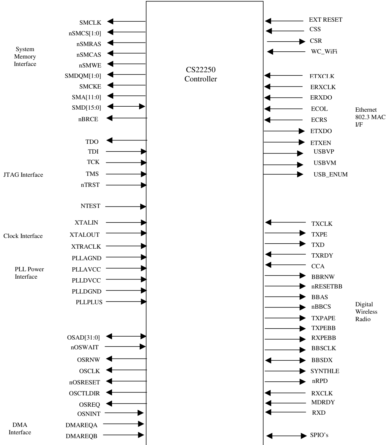
Figure 3. CS22250 Logical Pin Groupings
