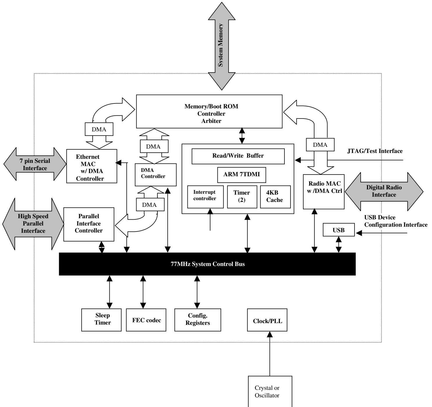
Figure 2. Block Diagram of Major Functional Units
