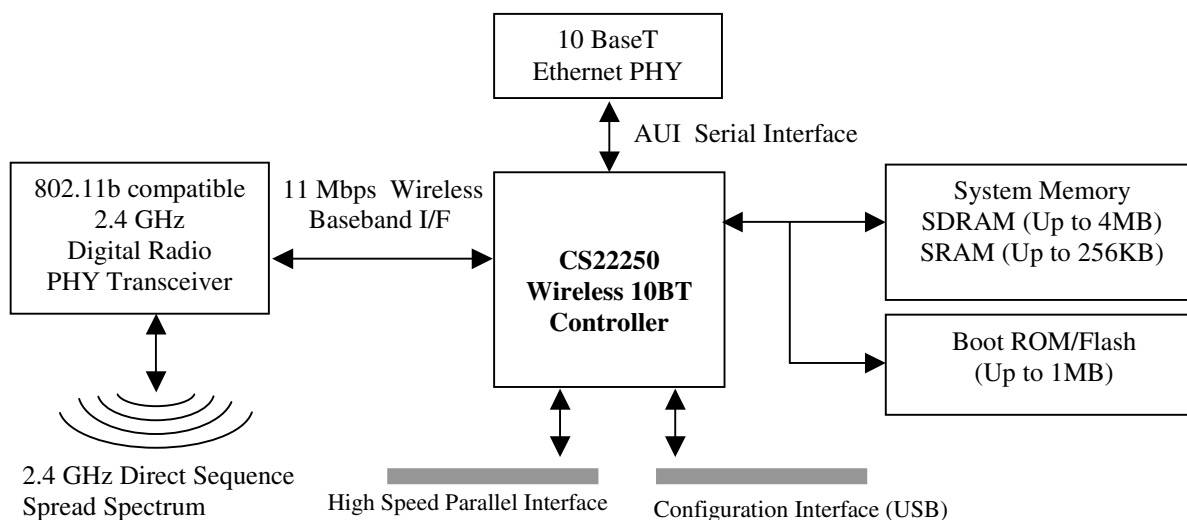
Figure 1. Example System Block Diagram
