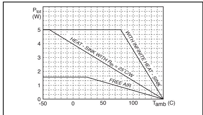
Figure 4 - Maximum Allowable Power Dissipation vs. Ambient Temperature for 16 lead fused package.
