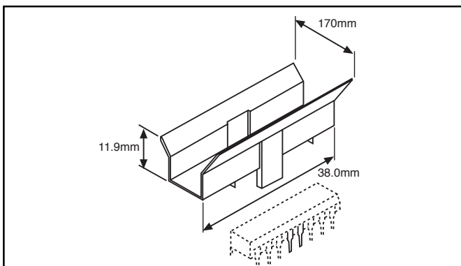
Figure 3 - External Heatsink Mounting Example ( R_{th} = 30^\circ C/W ) for 16 lead fused package.
