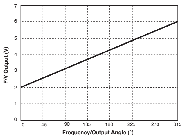
Figure 2: Charge Pump Output Voltage vs Output Angle
