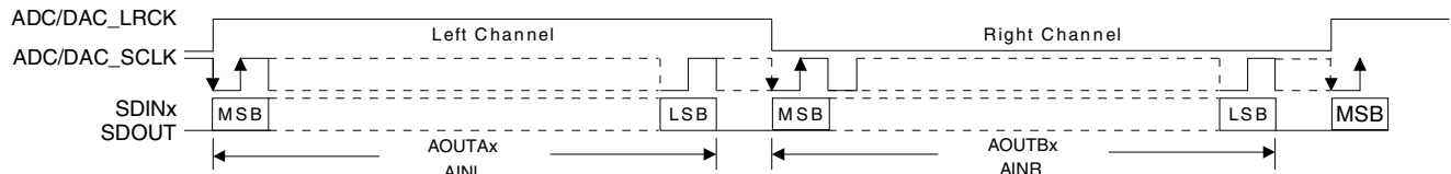
Figure 28. Left Justified up to 24-Bit Data
