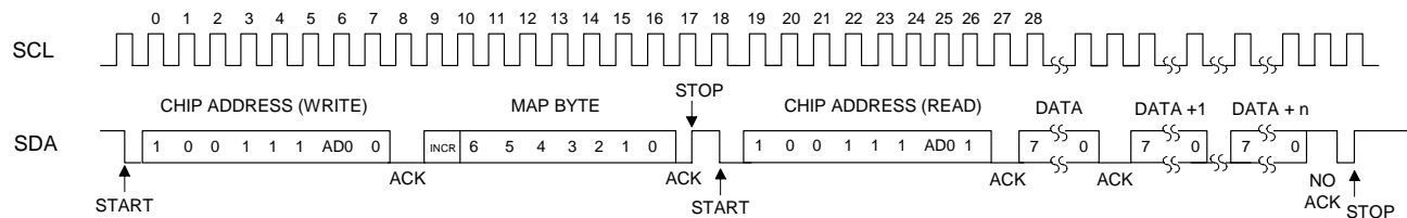
Figure 16. Control Port Timing, I²C Read
