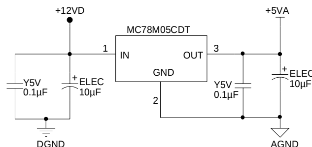
Figure 14. Voltage Regulator
