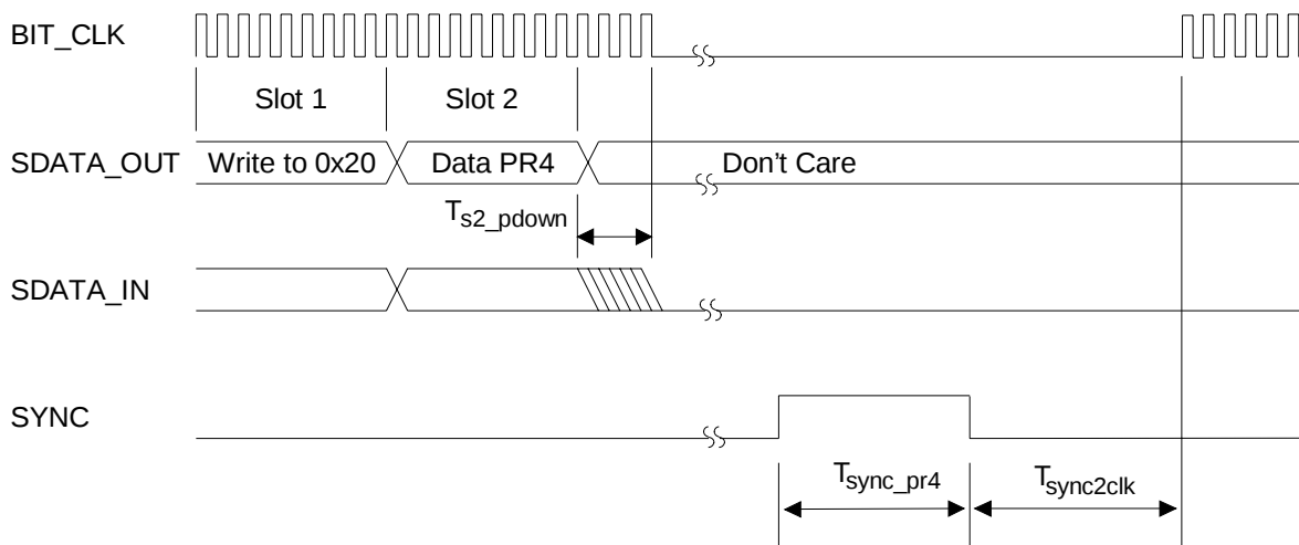
Figure 5. PR4 Powerdown
