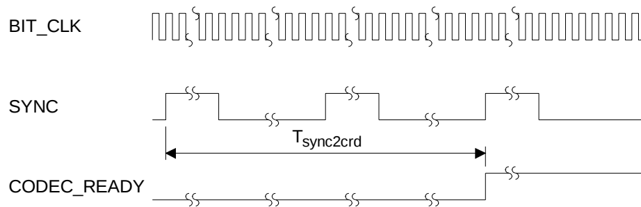
Figure 2. Clocks
