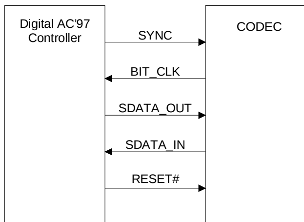
Figure 7. AC-link Connections
