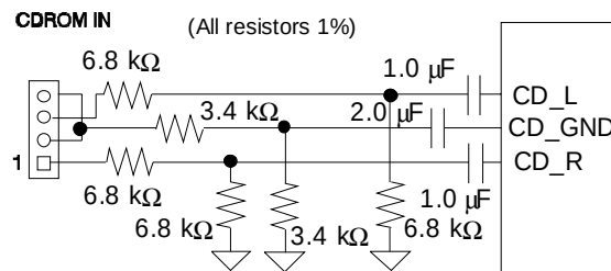
Figure 11. Differential CDROM In
