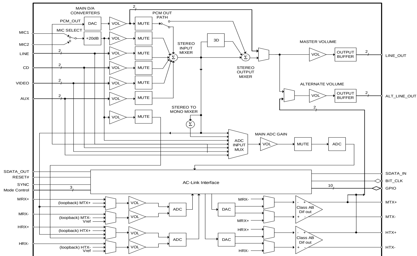
Figure 8. Mixer Diagram
