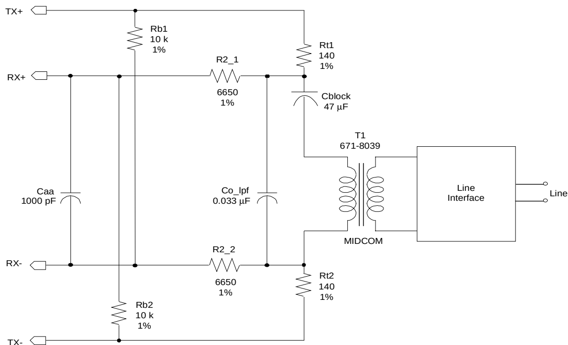
Figure 16. Hybrid Circuit Secondary
