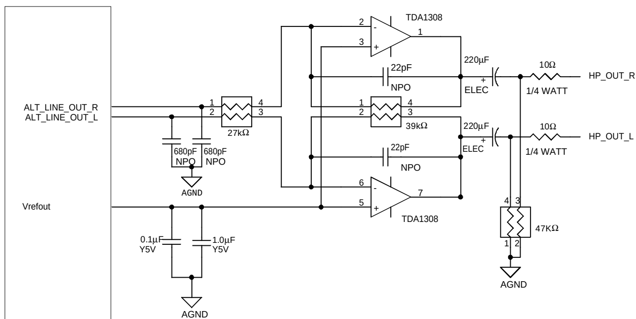
Figure 13. Headphones Driver
