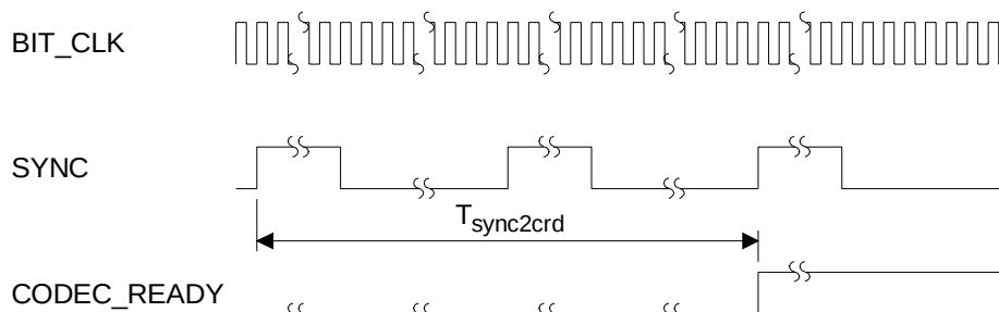
Figure 2. Clocks
