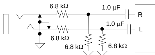
Figure 10. Line Inputs
