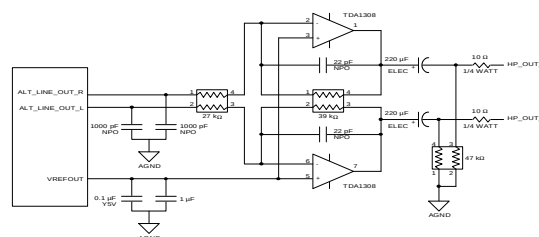
Figure 18. Stereo Output
