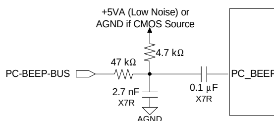
Figure 15. PC_BEEP Input
