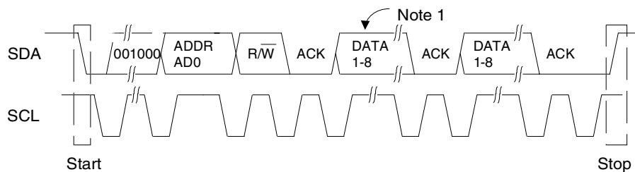
Figure 8. Control Port Timing, Two-Wire Format
