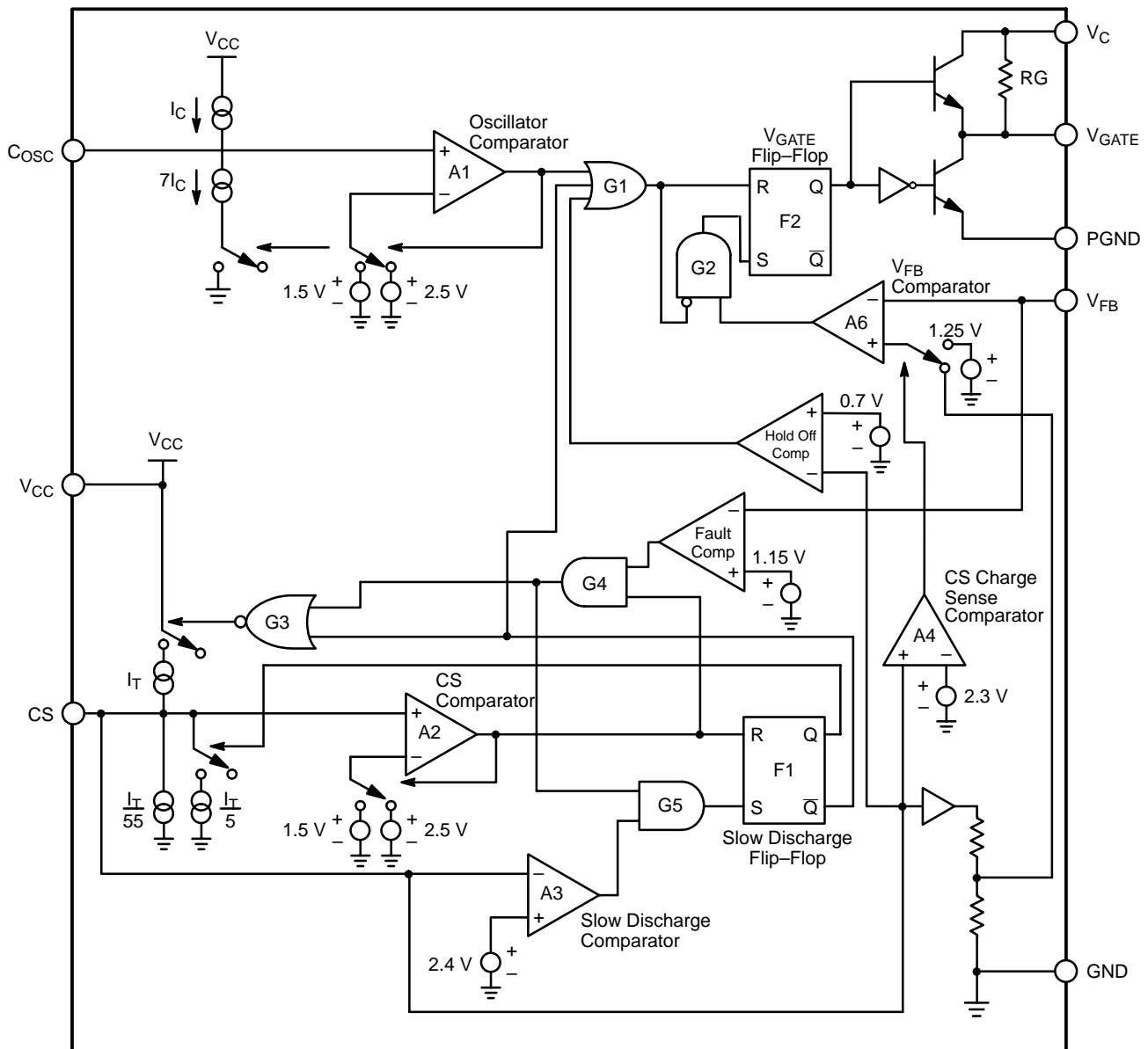
Figure 2. Block Diagram
