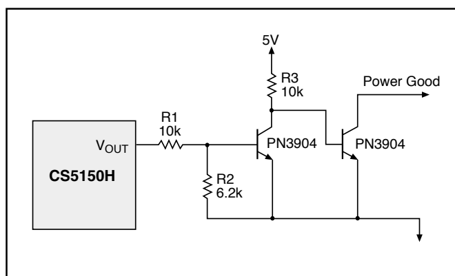
Figure 15: Implementing Power Good with the CS5150H.
