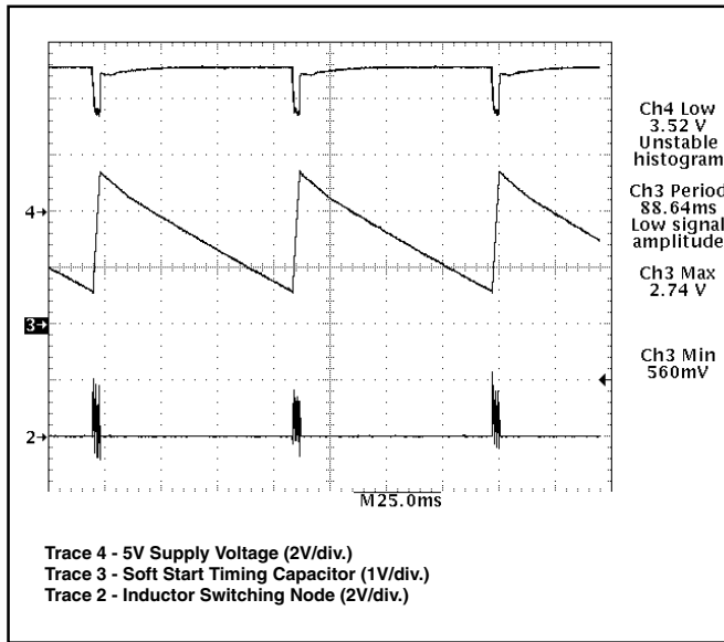
Figure 10: CS5150H demonstration board hiccup mode short circuit protection. Gate pulses are delivered while the soft start capacitor charges, and cease during discharge.
