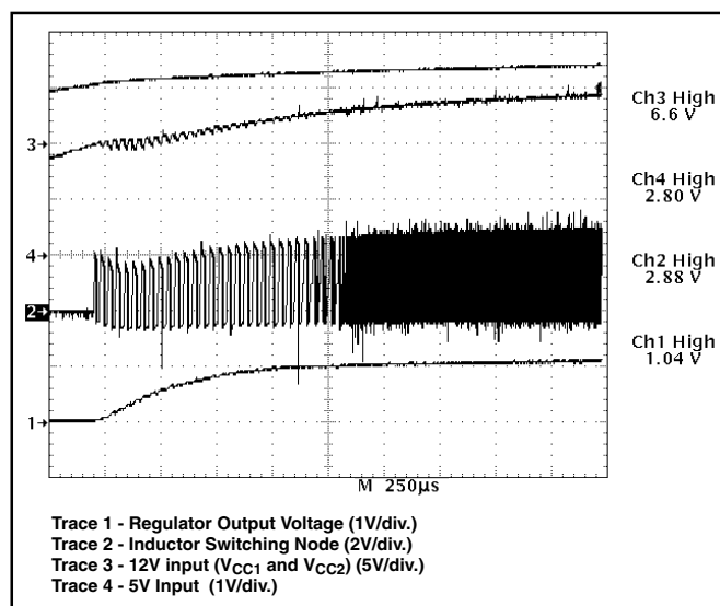
Figure 2: CS5151 demonstration board startup in response to increasing 12V and 5V input voltages. Extended off time is followed by normal off time operation when output voltage achieves regulation to the error amplifier output.
