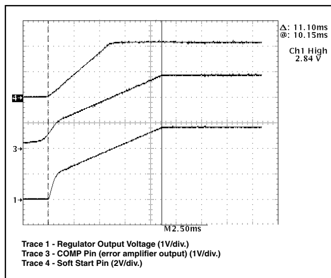
Figure 3: CS5151 demonstration board startup waveforms.
