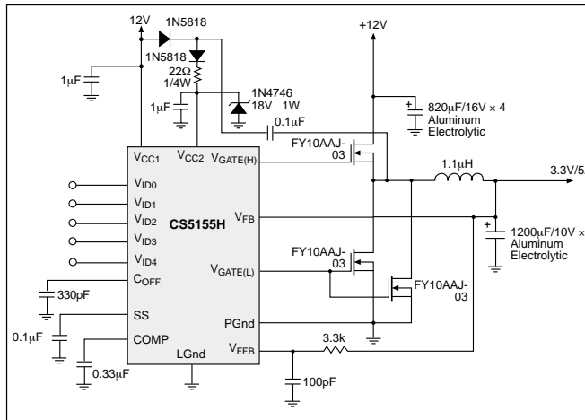
Figure 24: 12V to 3.3V/5A converter with remote sense.
