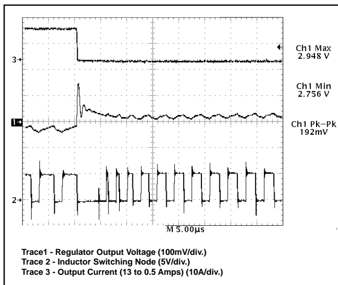
Figure 9: CS5157H demonstration board response to 13A load turn off (output set for 2.8V). V^{2TM} control topology immediately connects inductor to ground, providing 0% duty cycle. Regulation is achieved in less than 10μs.
