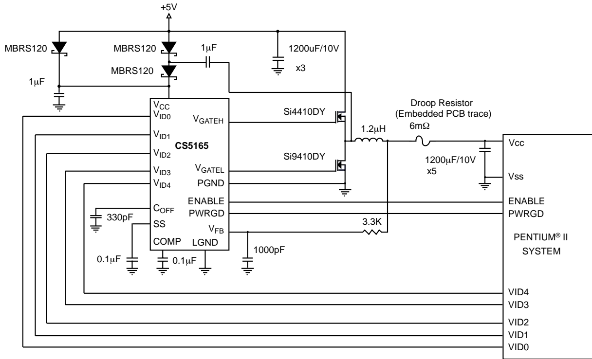
Figure 26: +5V to +2.8V @ 14.2A for 300 MHz PentiumII®
