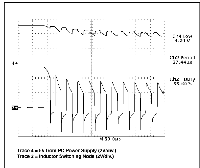
Figure 11: Demonstration board Start up with regulator output shorted to ground.
