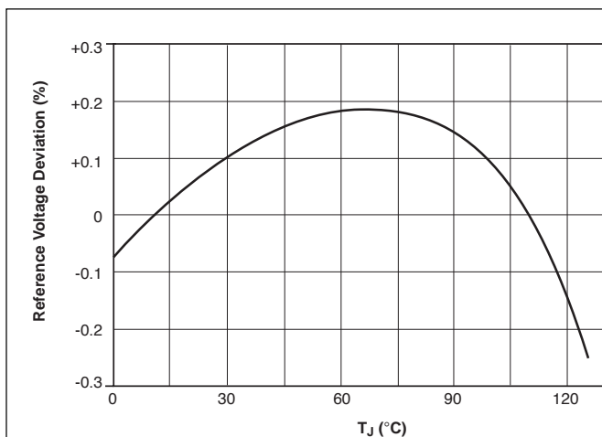
Output Voltage Deviation vs Temperature
