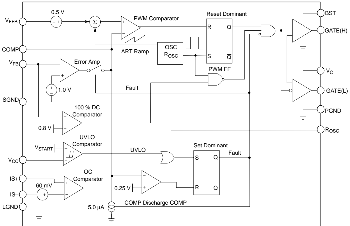
Figure 2. Block Diagram
