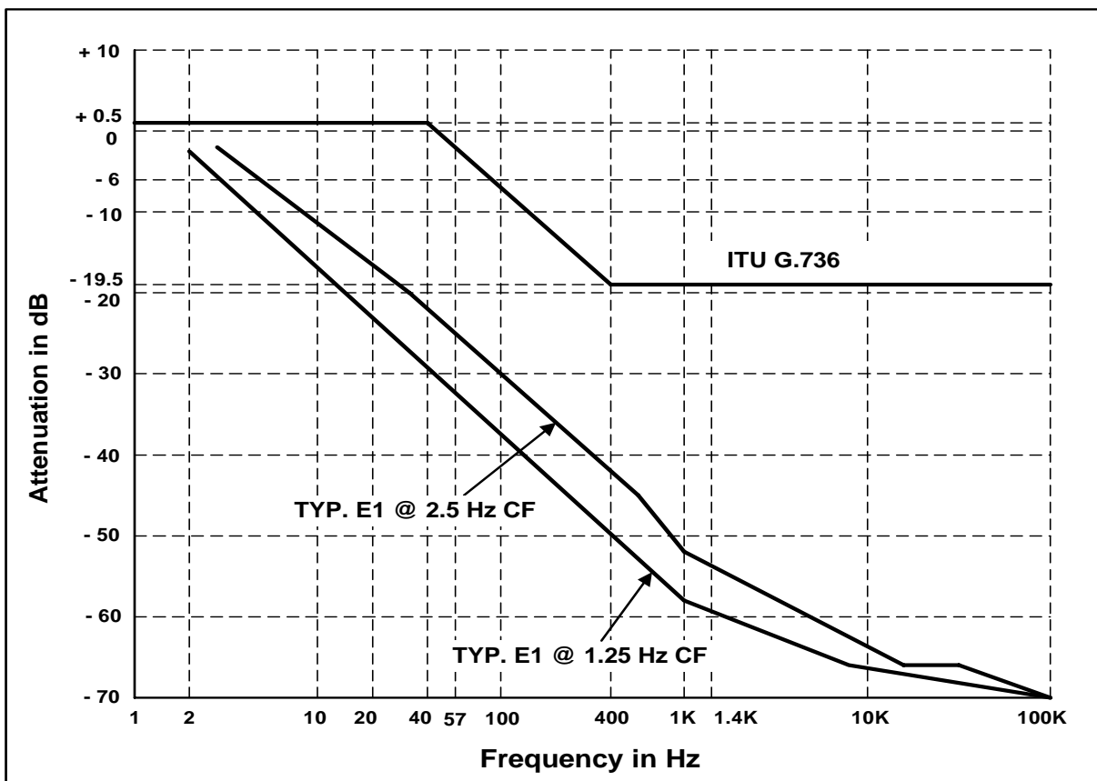
Figure 18. Jitter Transfer Characteristic vs. G.736 & TBR 12/13
