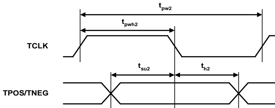
Figure 21. Transmit Clock and Data Switching Characteristics
