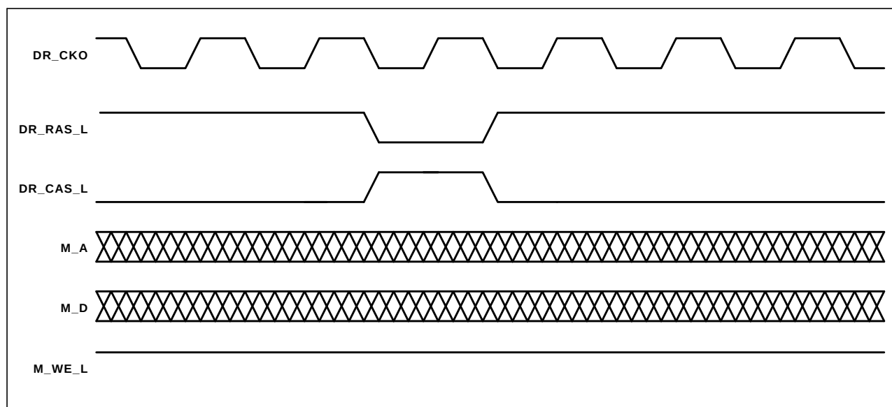
Figure 5. SDRAM Refresh
