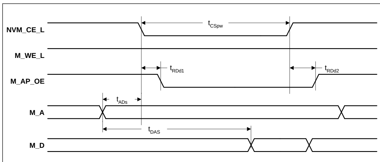
Figure 10. FLASH/ROM Read
