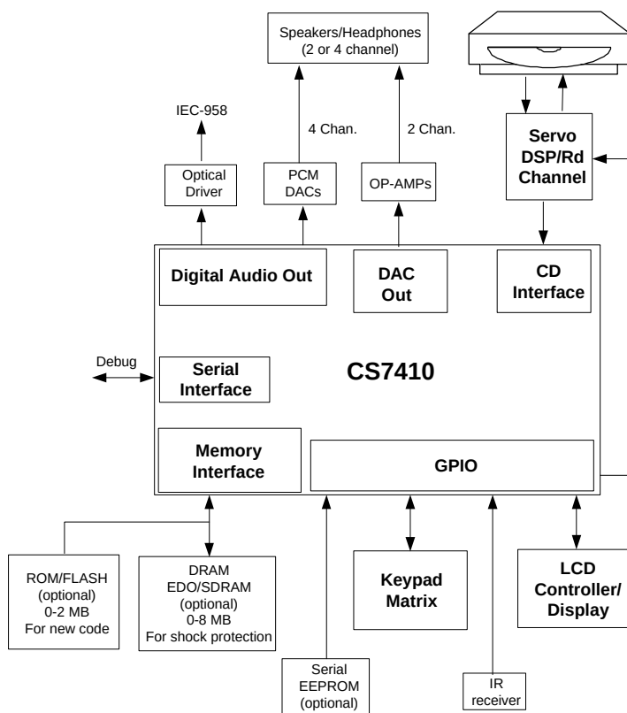
Figure 16. CS7410 Application
