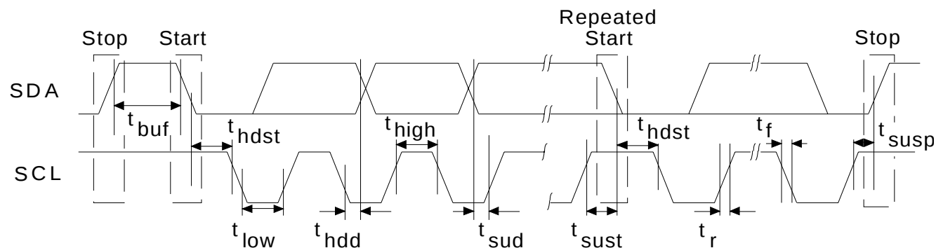
Figure 1. I²C Timing Diagram
