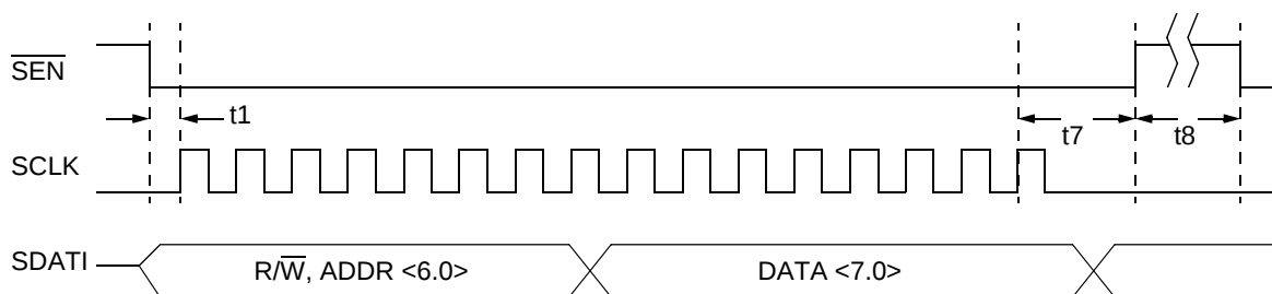
Figure 1. \overline{\text{SEN}} Timing
