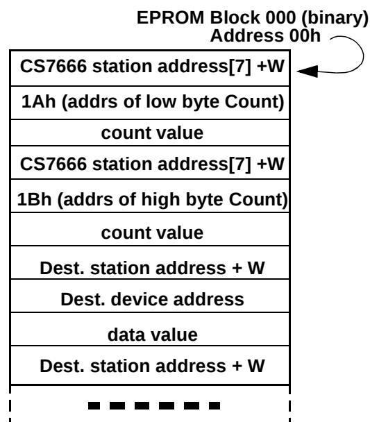
Figure 8. Map of EPROM table for initialization of registers
