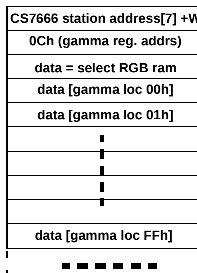
Figure 9. Map of EPROM table for storing gamma ram initialization data.
