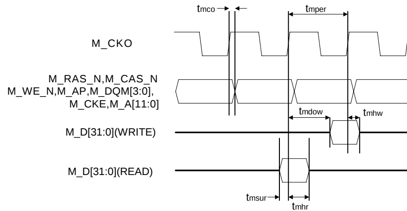
Figure 5. SDRAM Timing
