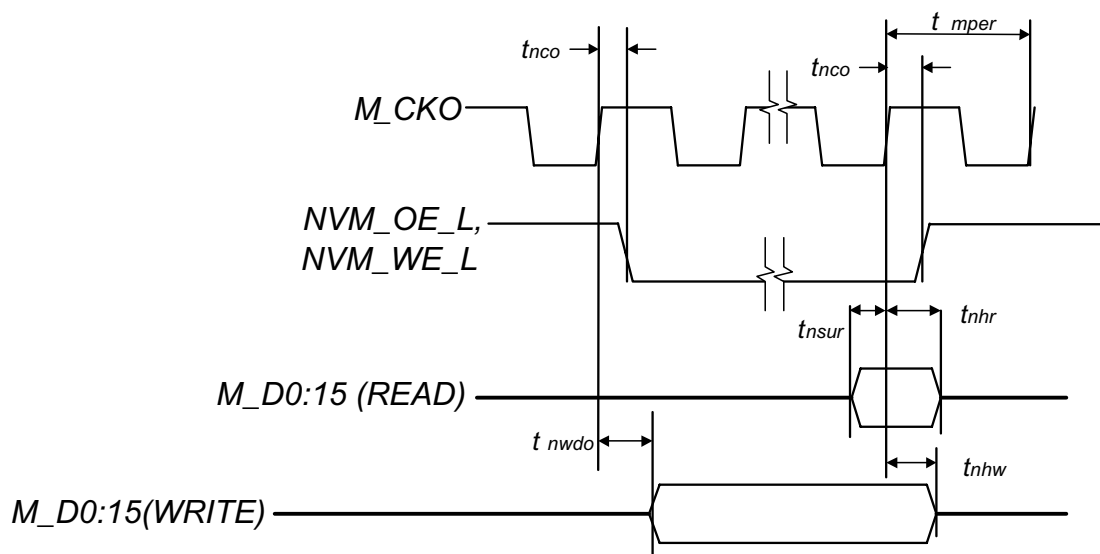
Figure 6. ROM/RVRAM Timing
