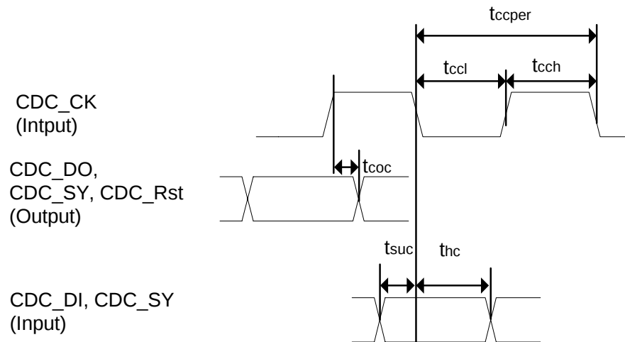
Figure 11. CODEC Timing
