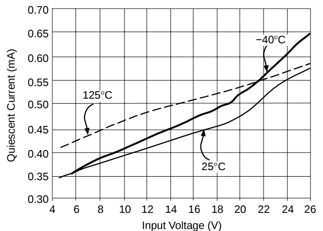
Figure 7. Quiescent Current vs. Input Voltage I_{OUT} = 100\text{ µA}
