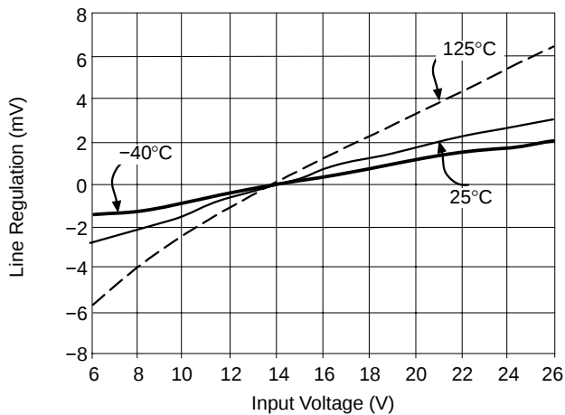
Figure 4. Line Regulation vs. Input Voltage I_{OUT} = 100\text{ µA}
