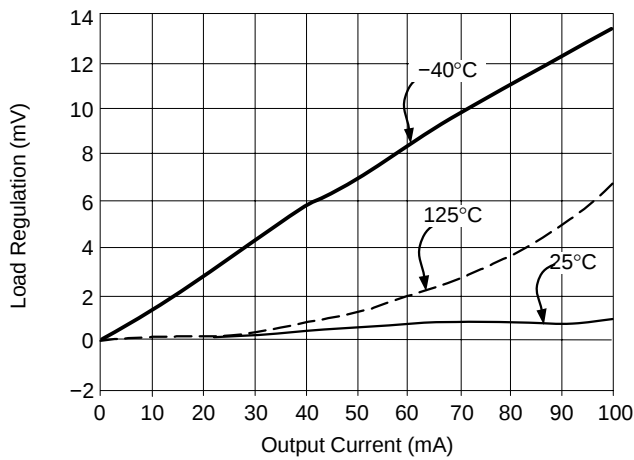
Figure 2. Load Regulation vs. Output Current V_{IN} = 14\text{ V}
