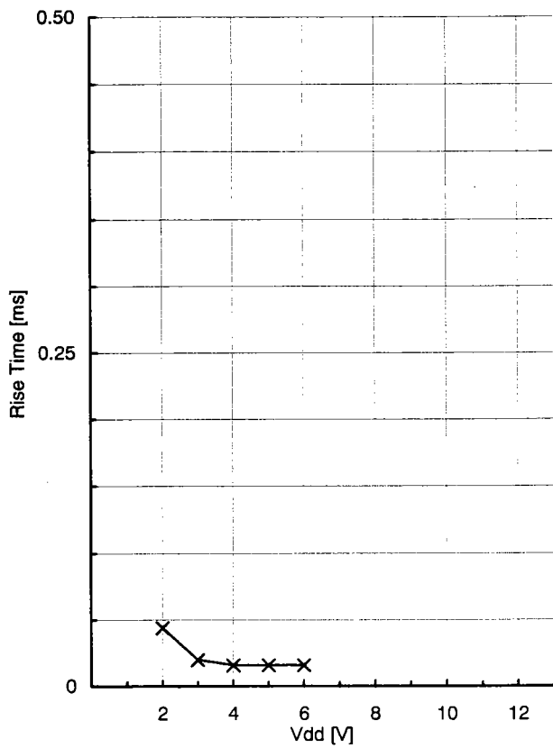
Rise Time vs Vdd Characteristics MODEL : CSTCC6.00MG with M34580E4
