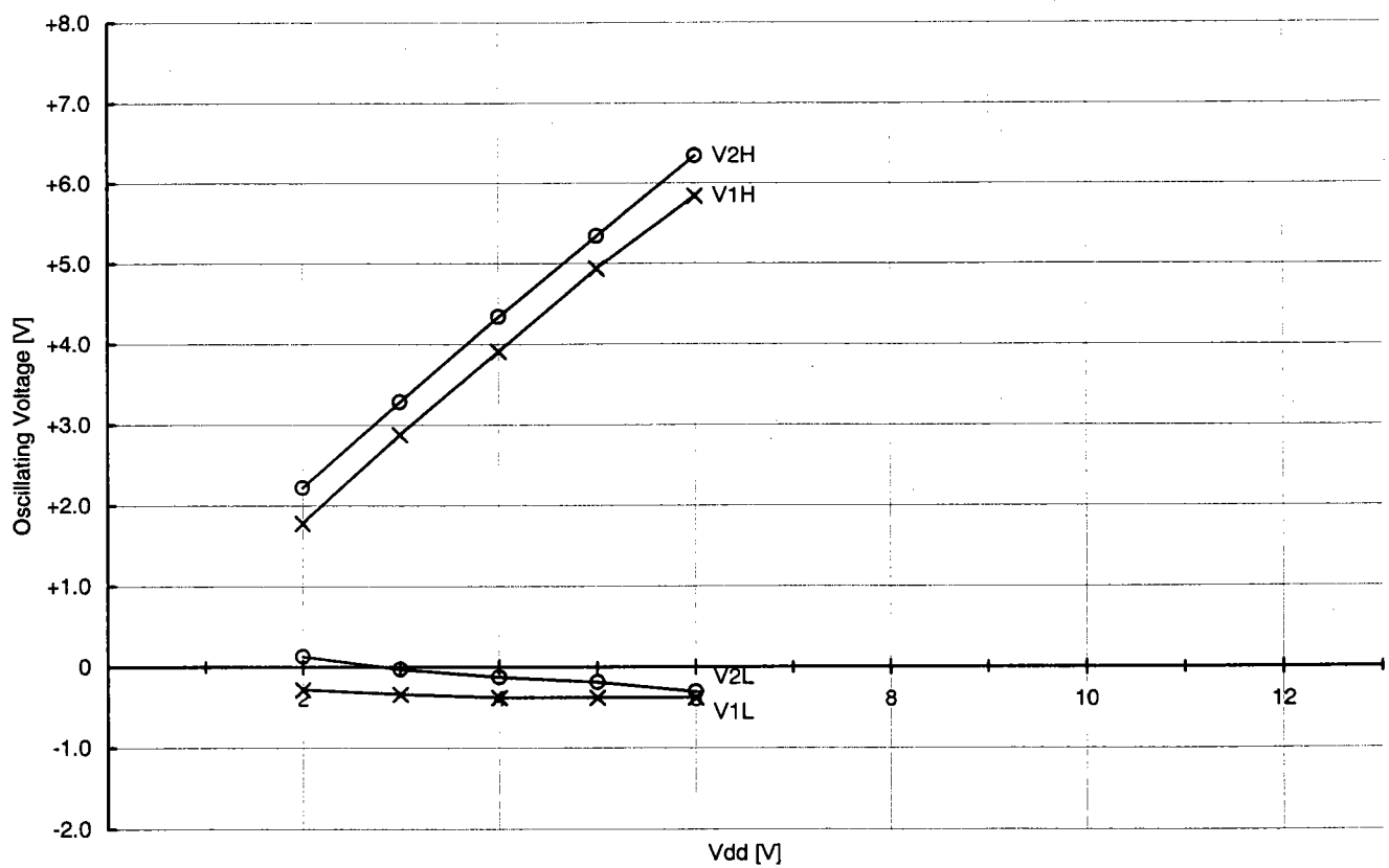
Oscillating Voltage vs Vdd Characteristics MODEL : CSTCC6.00MG with M34580E4
