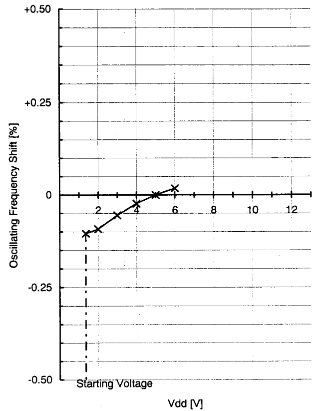
Oscillating Frequency vs Vdd Characteristics MODEL : CSTCC6.00MG with M34580E4
