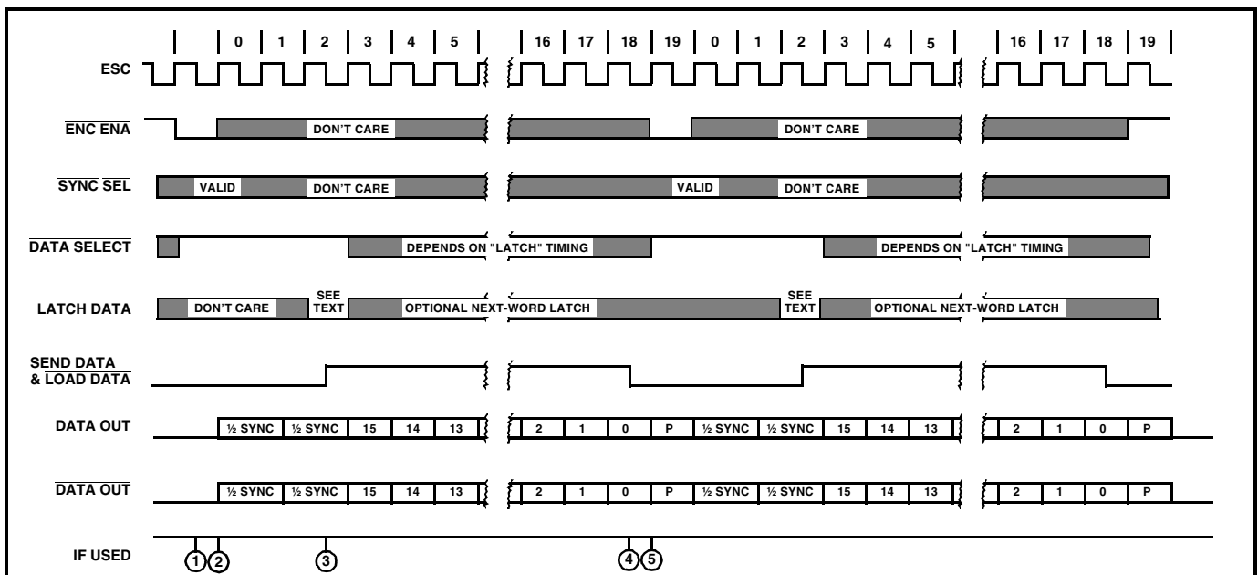
Figure 3 – Transmit Cycle Timing
