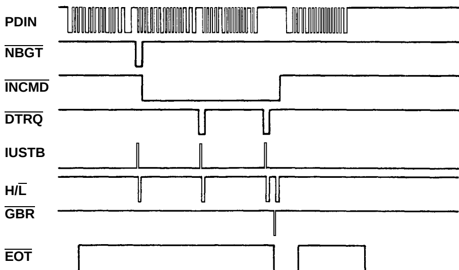
Figure 7 – Transfer of two Data Words from BC to RT 03
