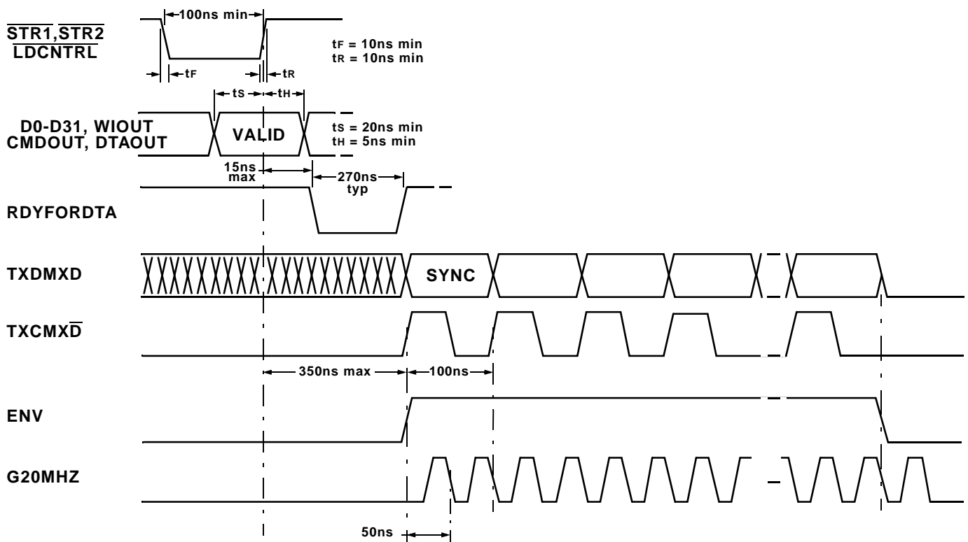
Figure 2 – Transmit Timing Diagram
