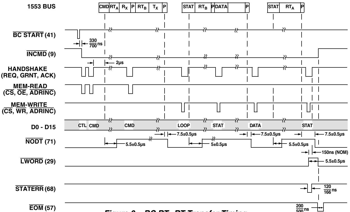
Figure 9 – BC RT-RT Transfer Timing
