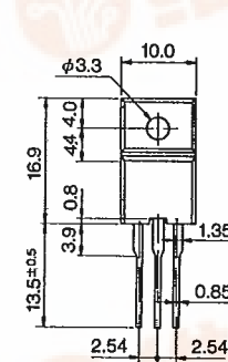
Outline Drawing ④⑦
