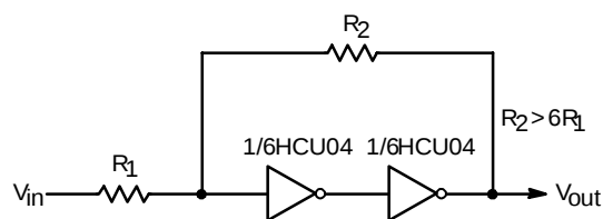
Schmitt Trigger
