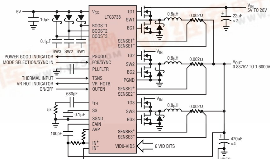
VRM10 Step-Down Controller
