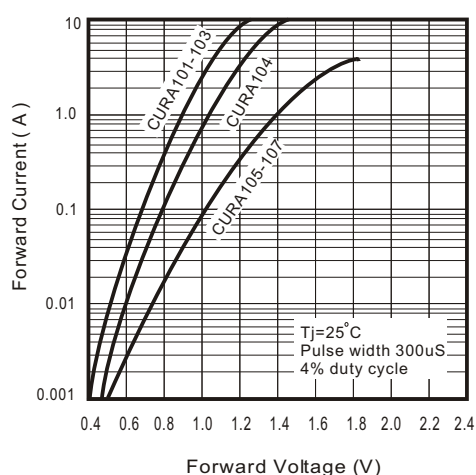
Fig.2 - Forward Characteristics
