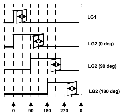
FIGURE 4. PHASE OF LG2 WITH RESPECT TO RISING EDGE OF LG1
