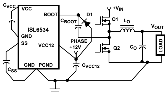
FIGURE 22. PRINTED CIRCUIT BOARD SMALL SIGNAL LAYOUT GUIDELINES
