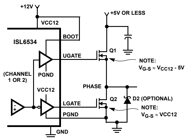
FIGURE 18. UPPER GATE DRIVE - DIRECT VCC12 DRIVE OPTION
