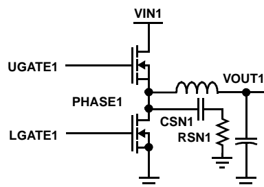
FIGURE 19. SNUBBER COMPONENT SELECTION
