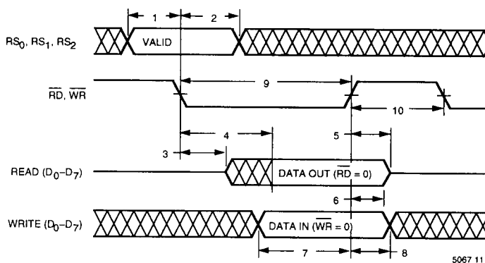
Figure 7. MPU Read/Write Timing
