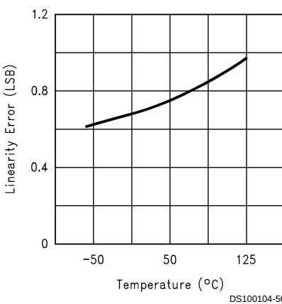
Linearity Error vs Temperature
