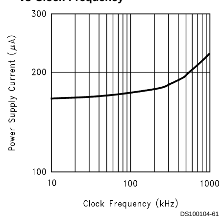
Power Supply Current vs Clock Frequency
