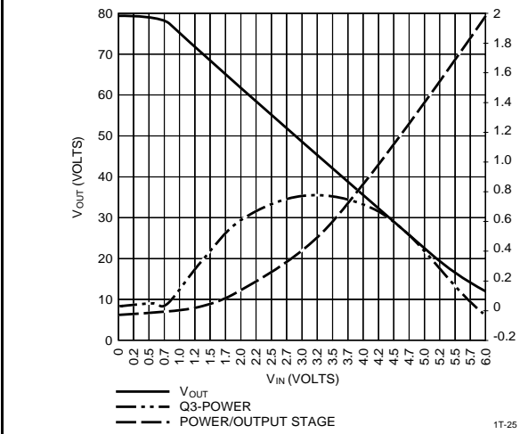
FIGURE 1. CVA1775N DC CHARACTERISTICS
