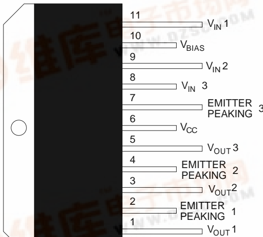
TOP VIEW T11A PACKAGE
