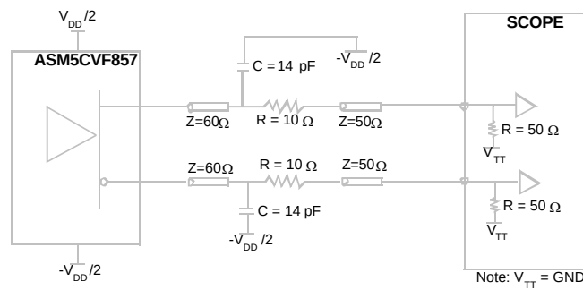
Figure 2: Output Load Test Circuit
