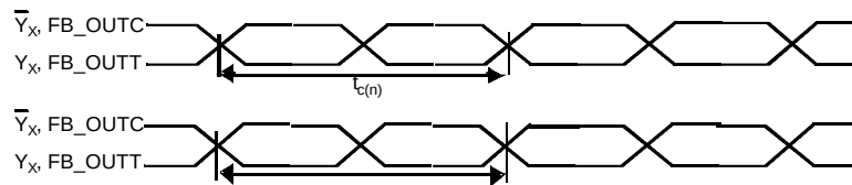
Figure 7: Period Jitter
