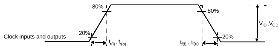
Figure 9: Input and Output Slew rates
