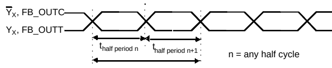
Figure 8: Half-Period Jitter
