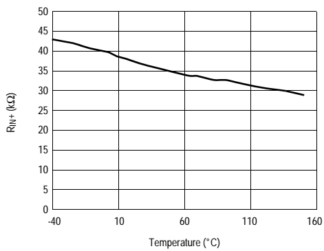
Positive Input Resistance vs Temperature
