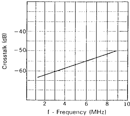
CH-2 → CH-1 crosstalk with PB RF output 2 vs. Frequency
