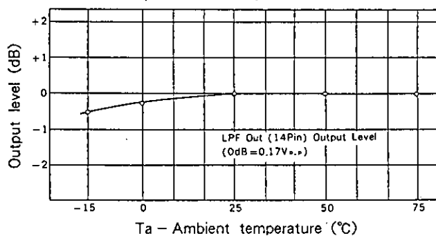
Modulator output level temperature characteristics
