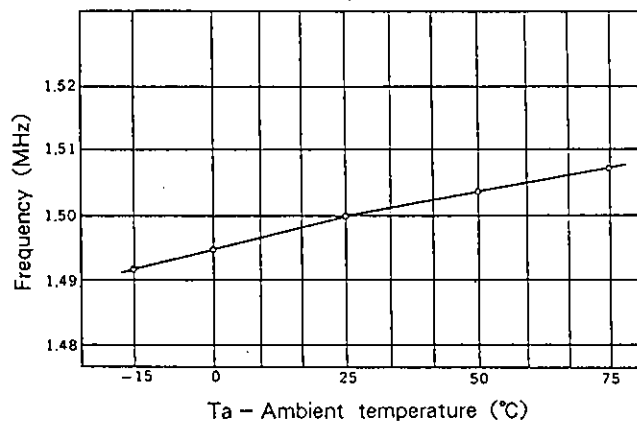
Modulator carrier temperature characteristics
