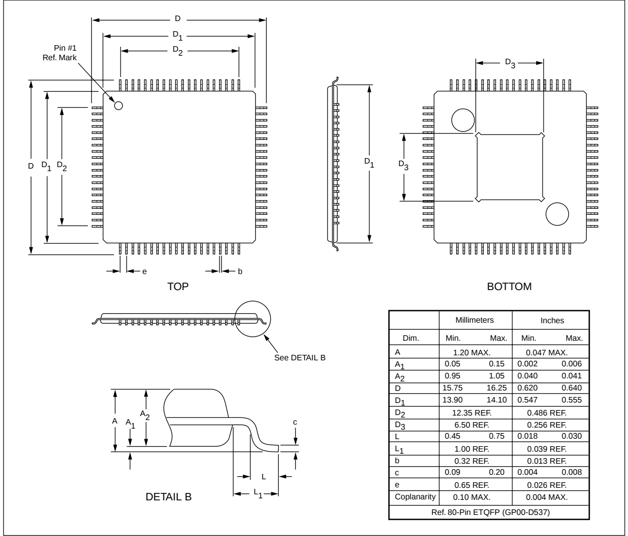
Figure 2-10. CX2833i-1x Mechanical Drawing (80-Pin)—Dimensions
