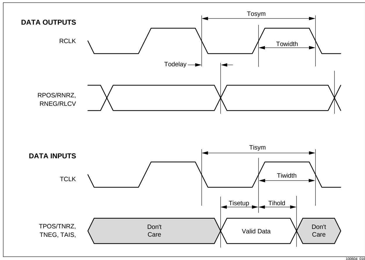
Figure 2-12. Timing Diagram
