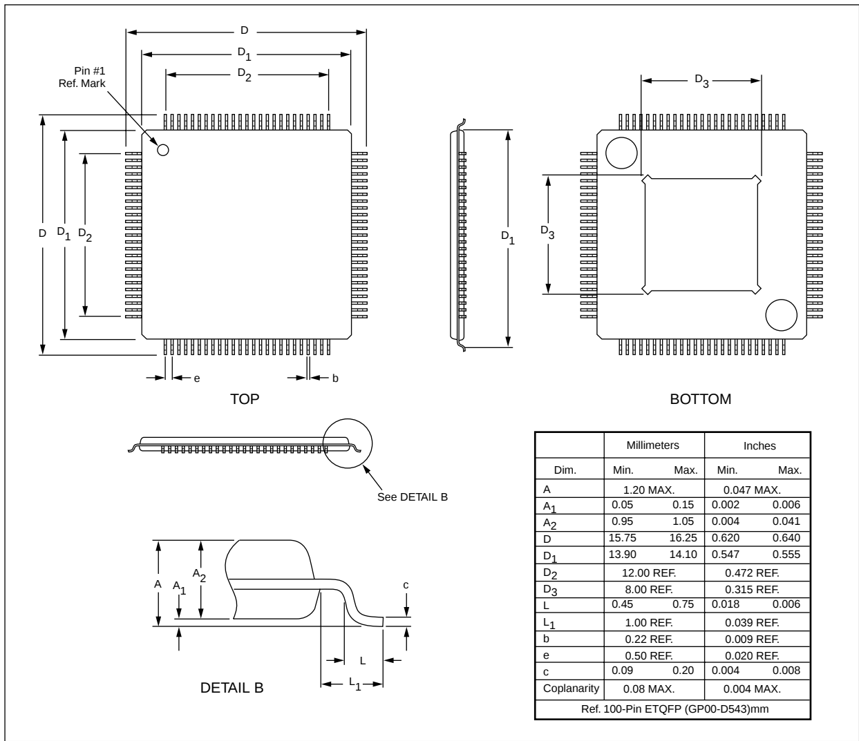
Figure 2-11. CX28331-3x Mechanical Drawing (100-Pin)—Dimensions
