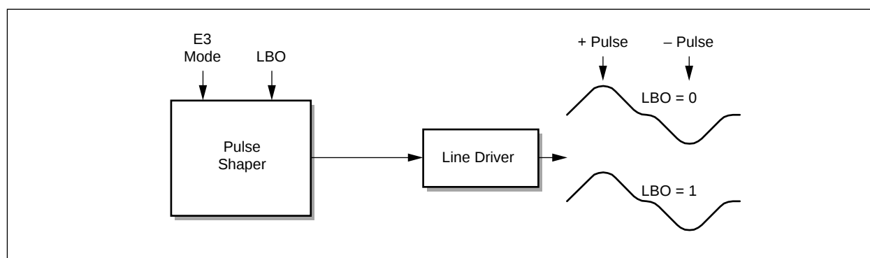
Figure 2-2. Pulse Shaper
