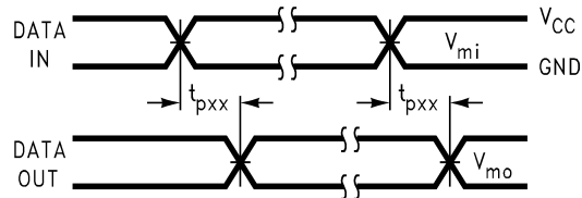
FIGURE 8. Waveform for Inverting and Non-Inverting Functions
