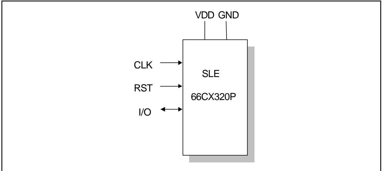
Figure 1 Pin Configuration
