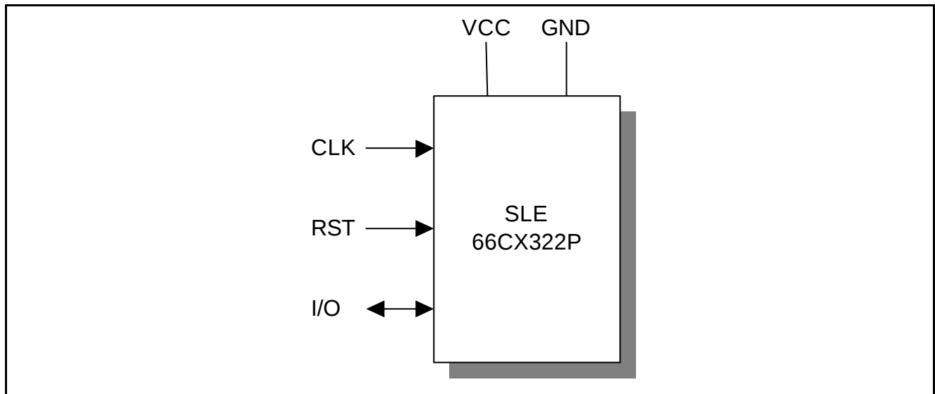
Figure 1: Pin Configuration
