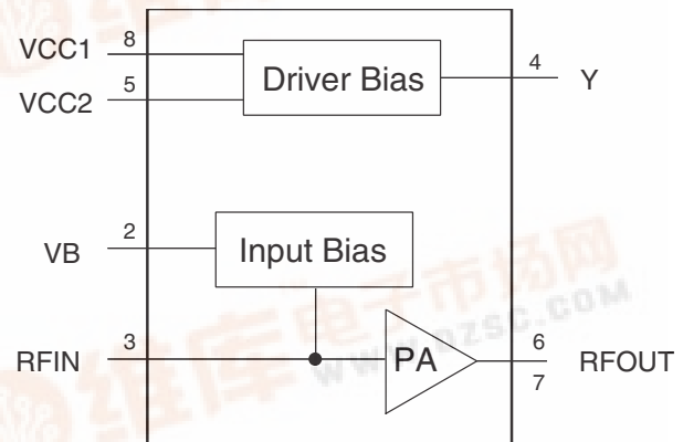
Figure 2. CX65002 Functional Block Diagram
