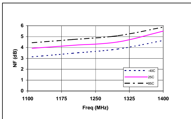
Figure 10. Typical NF From 1.1 to 1.4 GHz Over Temperature (Circuit Match for Optimum Gain)
