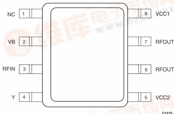
Figure 1. CX65002 Pinout – 8-Pin SOIC Package (Top View)
