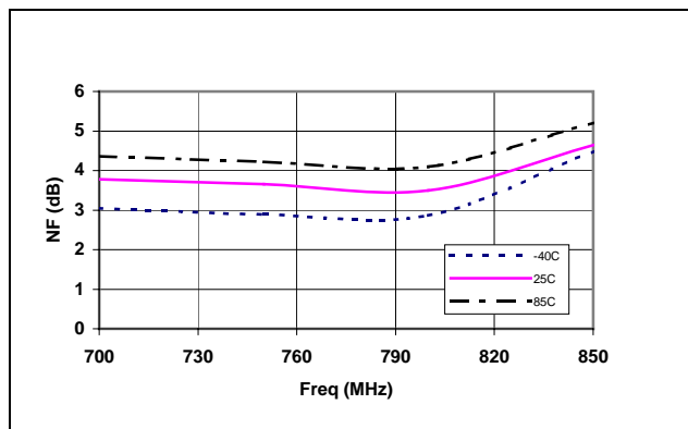
Figure 8. Typical NF From 700 to 850 MHz Over Temperature (Circuit Match for Optimum Gain)
