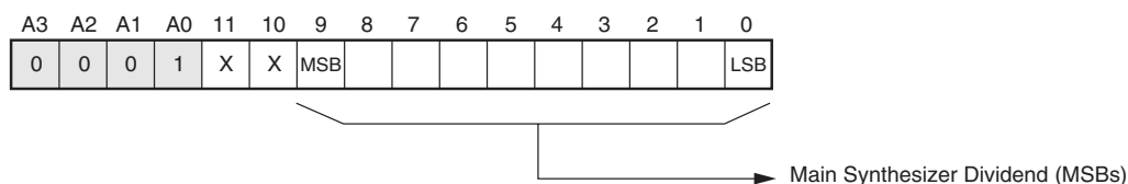
Figure 7. Main Dividend MSB Register (Write Only)
