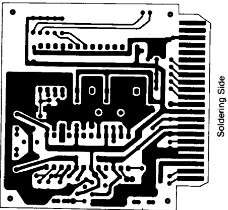
CX20052A PCB-3A/3B Pattern
