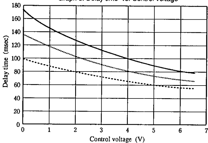
Graph 3. Delay time vs. Control voltage
